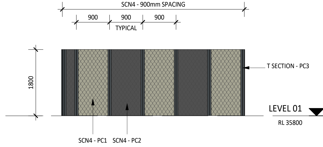
6 REFRIGERATION WORKSHOP BALCONY SCREEN 44-05 1 : 50
