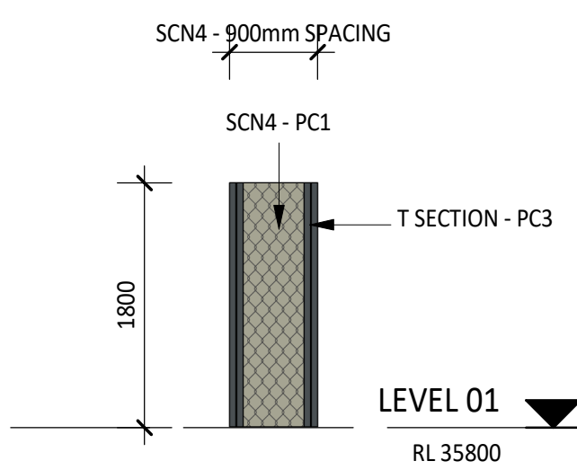
7 REFRIGERATION WORKSHOP BALCONY SCREEN 44-05 1 : 50
