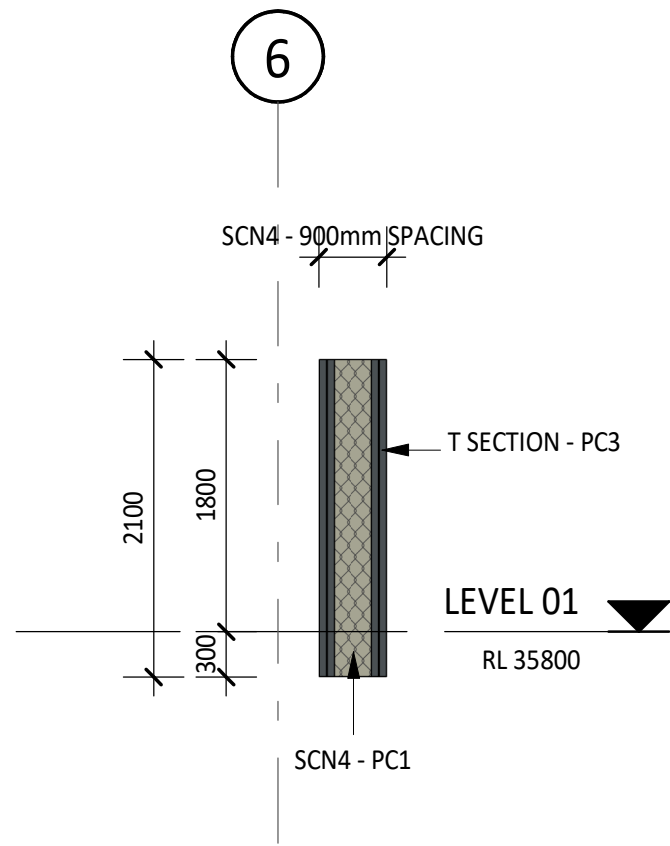
3 REFRIGERATION WORKSHOP BALCONY SCREEN 44-05 1 : 50
