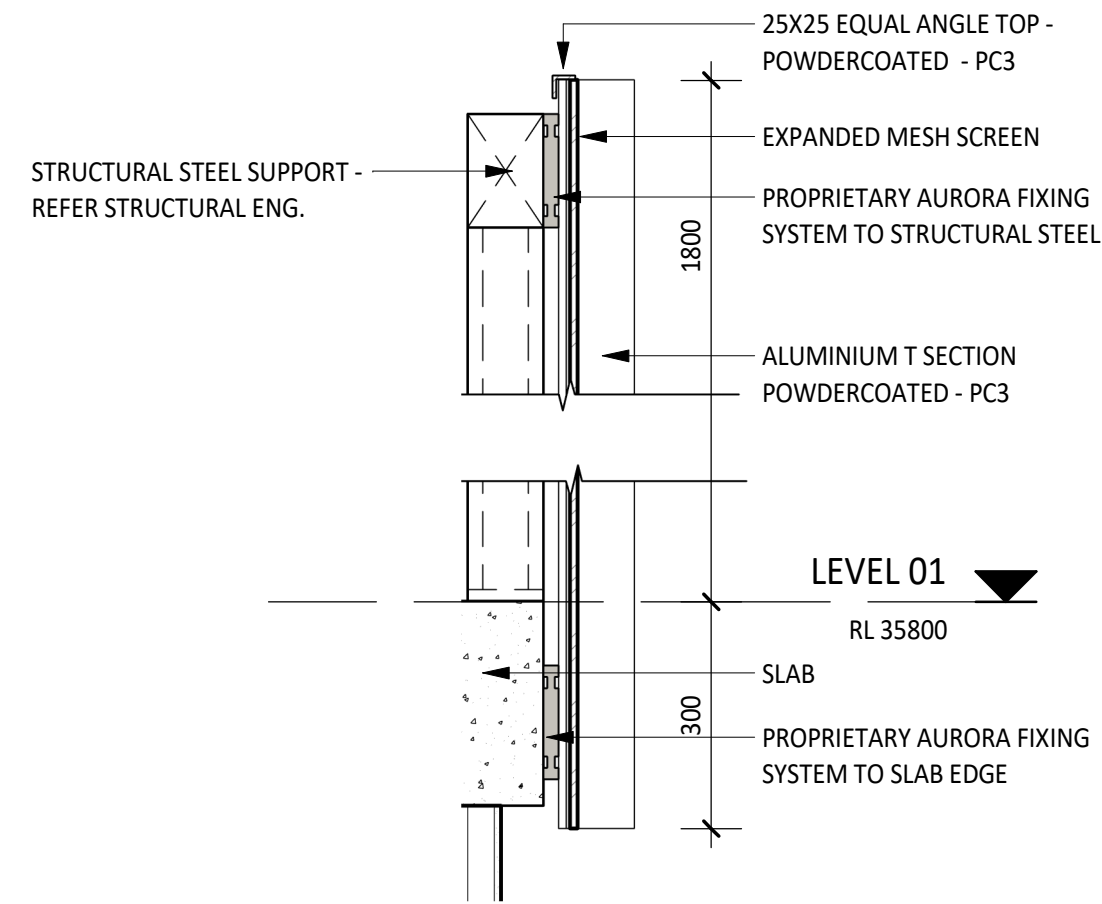
10 DETAIL SCN4 BALUSTRADE - TYPICAL SECTION 44-05 1 : 10
