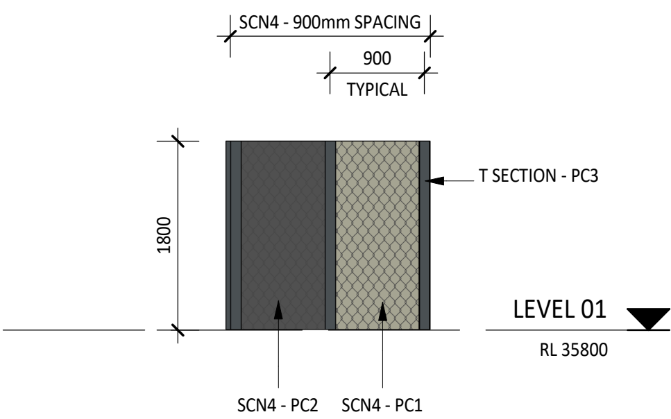
5 REFRIGERATION WORKSHOP BALCONY SCREEN 44-05 1 : 50
