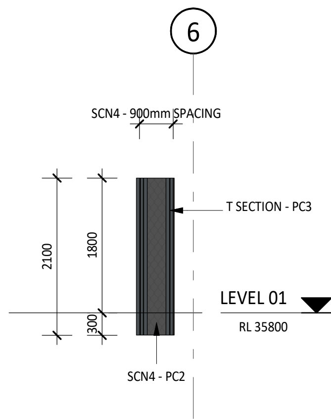
4 REFRIGERATION WORKSHOP BALCONY SCREEN 44-05 1 : 50
