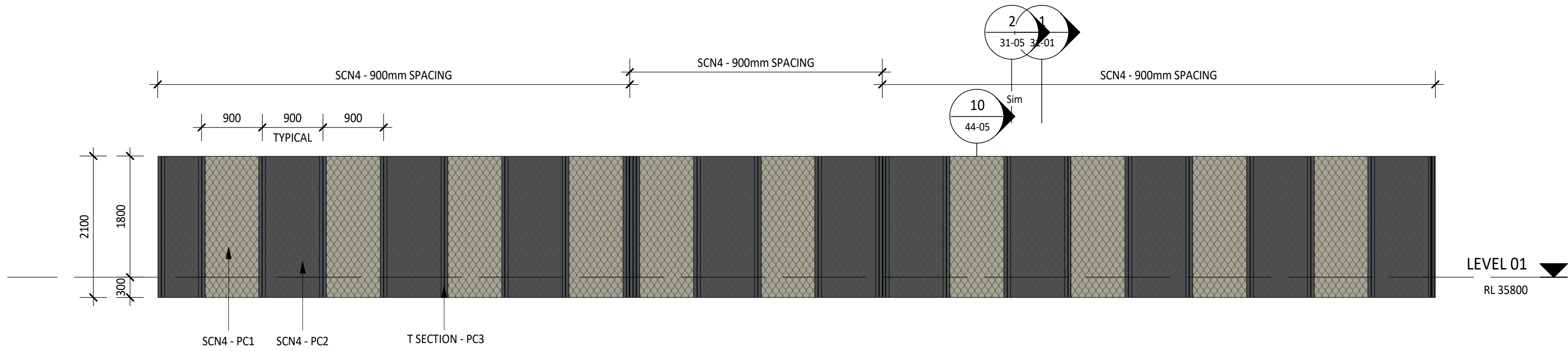
2 REFRIGERATION WORKSHOP BALCONY SCREEN 44-05 1 : 50
